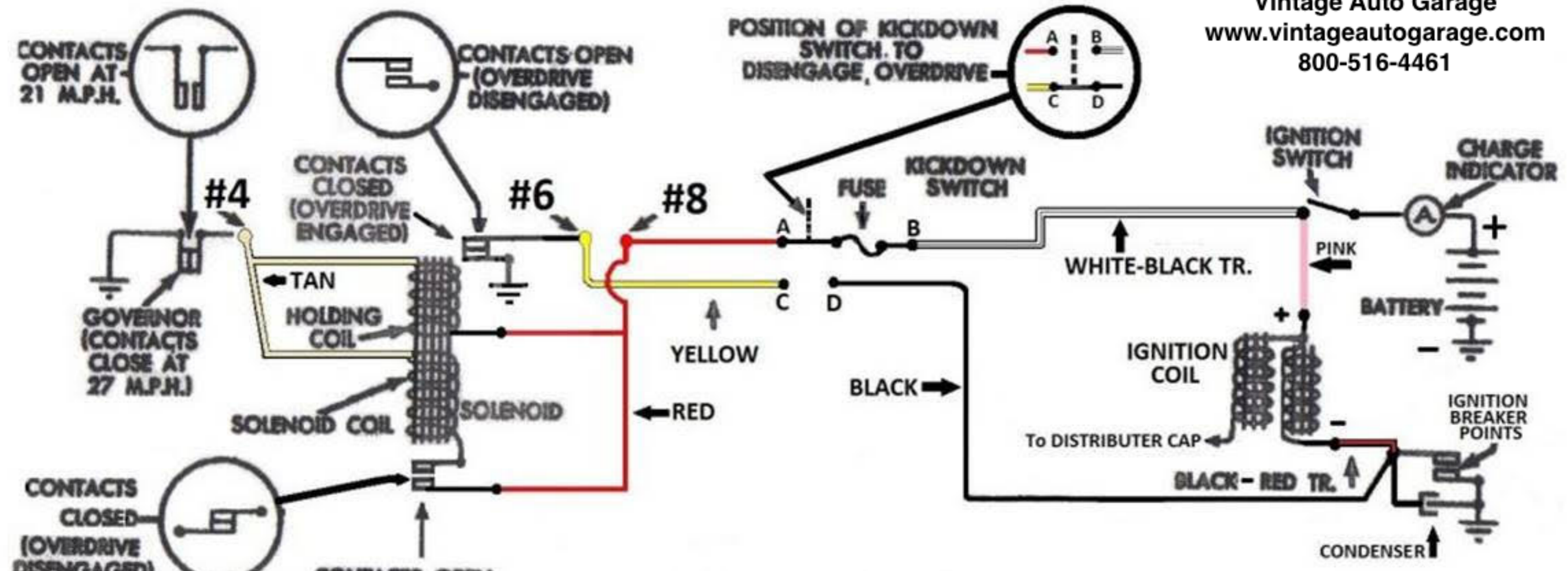
OVERDRIVE ELECTRICAL CIRCUIT 1962 STUDEBAKER GRAN TURISMO HAWK
